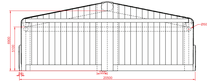
SIDE ELEVATION
