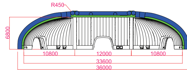
SECTION VIEW
