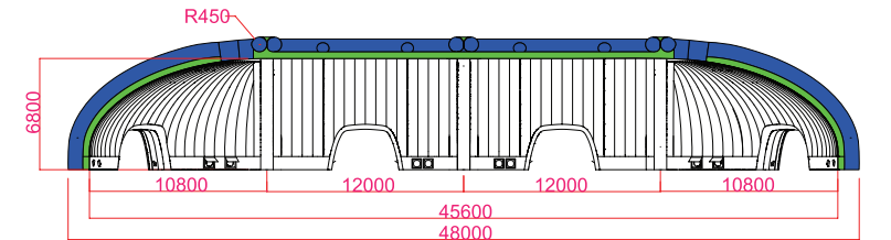
SECTION VIEW
