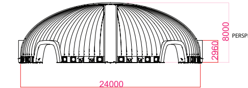
FRONT
