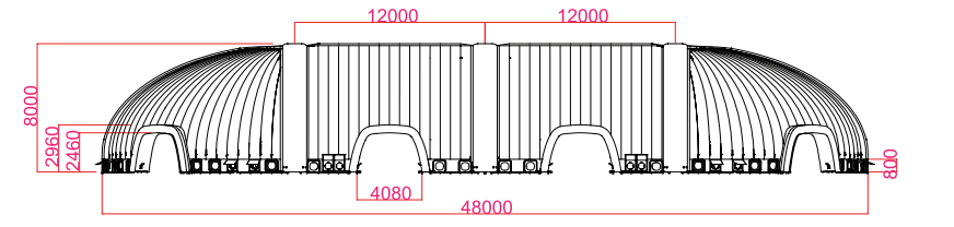
SIDE
