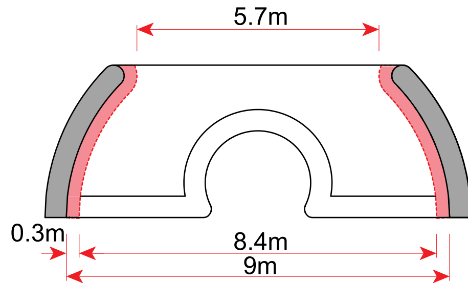
SECTION AA - EXCLUSION ZONE SHARP OBJECTS SHOULD NOT BE PLACED IN THIS ZONE
