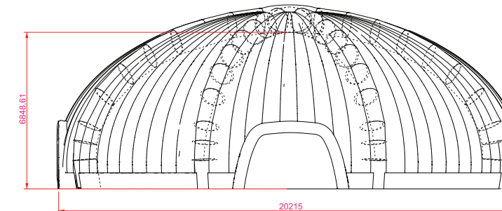
FRONT ELEVATION
